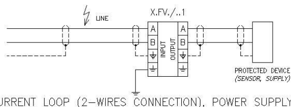
CURRENT LOOP (2-WIRES CONNECTION), POWER SUPPLY
